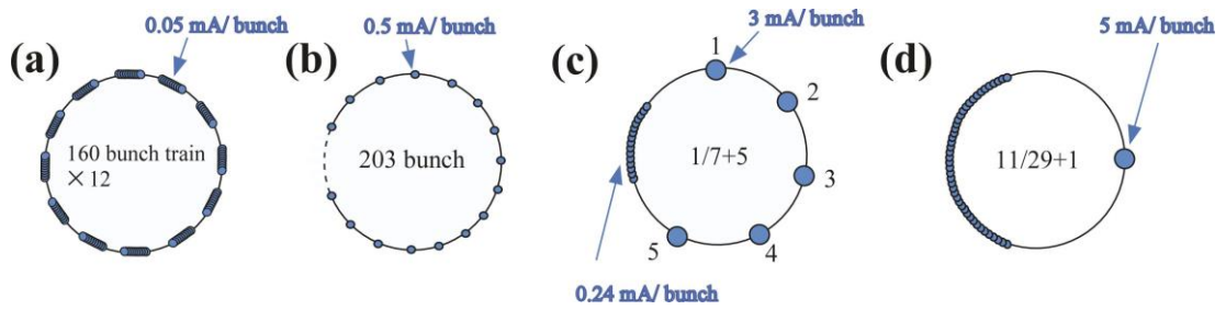
Fig.4 Examples of the filling patterns of electron bunches in the storage ring.
